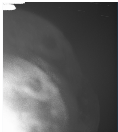
Figure 3: Maximum-Stacked Lunar Image Obtained from a Sequence of Registered Frames Affected by Tracking Inaccuracies. Misalignment Results in Duplicated Lunar Features and Prevents Reliable Detection of Localized Transients.
