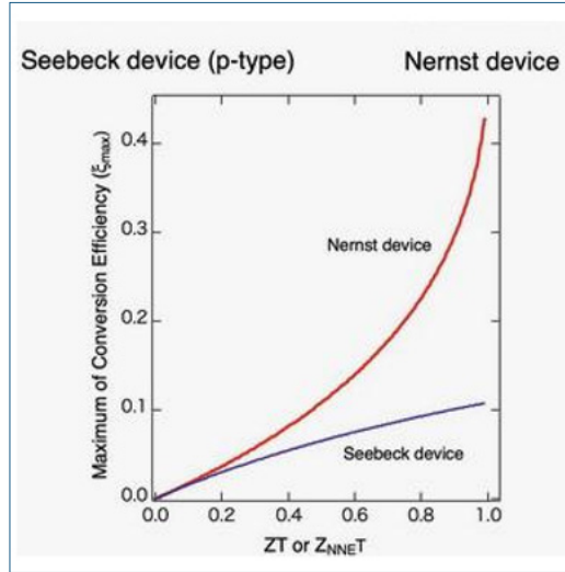
Figure 1: The Dependence of the Efficiency of Thermoelectric Voltage Generation on the Parameters a ZT and Z_{NNE}T for the Seebeck Effect and the Nernst Effect.
